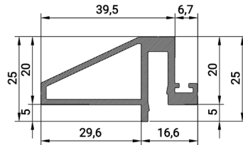
FS 3229 SINGLE RAIL WALL COVER WEIGHT 0.682 KG/M
