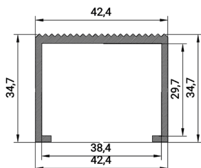
FS 3247 SILL PROFILE WEIGHT 0.850 KG/M
