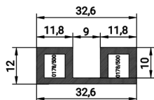
FS 3254 SINGLE GLASS ADAPTOR WEIGHT 0.526 KG/M
