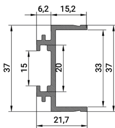
FS 3210 LATCHING HANDLE PROFILE POLYCARBONATE
