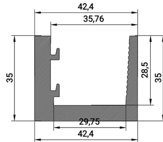
BP 002.1 BALAUSTRADE SILL PROFILE WEIGHT 0.634 KG/M
