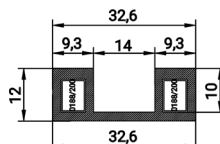
FS 3248 SINGLE GLASS ADAPTOR WEIGHT 0.450 KG/M
