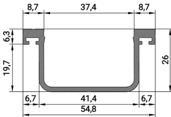
FS 3225 SINGLE RAIL INTERLOCK WEIGHT 0.631 KG/M
