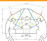
Alu-Round profile with 30° lens LEDs type 3528
