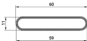
FS 3261 DRAINAGE BOX PIPE WEIGHT 0.411 KG/M
