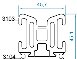
code : 3103 +3104 كانكتور كشویی Transom Joint Profile weight :2.3+0.48kg/m
