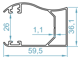
ریل نایس Nice Rail Profile code: 9154
