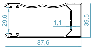
ریل کستل Castle Rail Profile code: 9151
