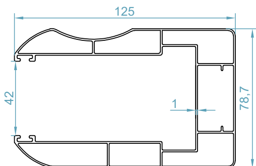
ریل جاینٹ Giant Rail Profile code: 9156
